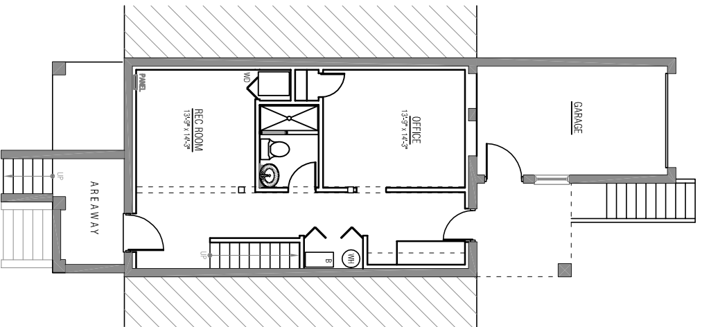
BASEMENT
